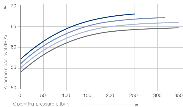
IPVS 5 – Airborne noise level (measuring point 1 m axial)
