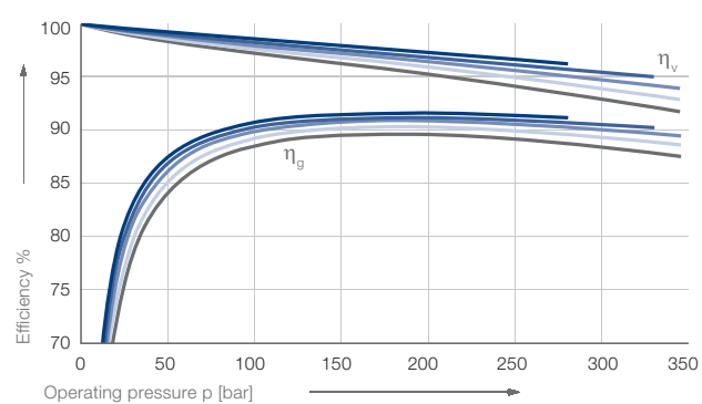
IPVS 4 – Efficiency \eta_v and \eta_g
