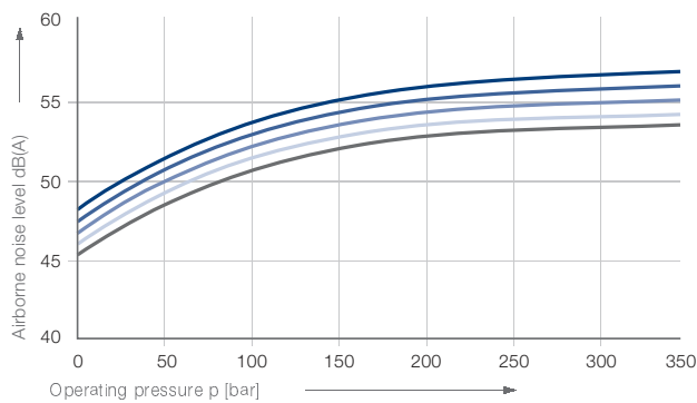
IPVS 3 – Airborne noise level (measuring point 1 m axial)
