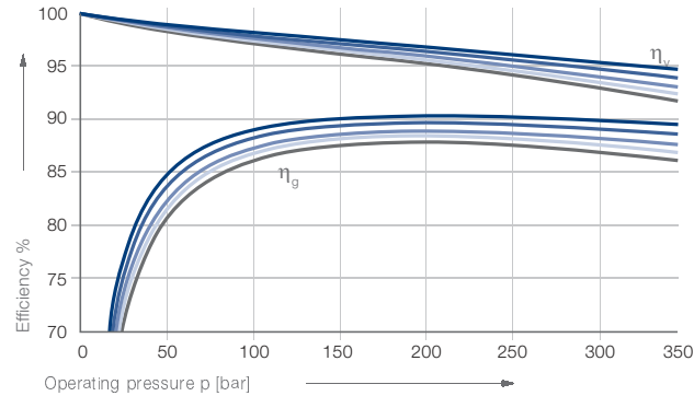
IPVS 3 – Efficiency \eta_v and \eta_g
