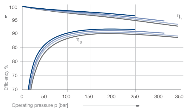
IPVS 5 – Efficiency \eta_v and \eta_g
