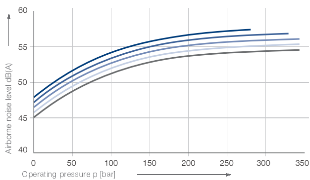
IPVS 4 – Airborne noise level (measuring point 1 m axial)
